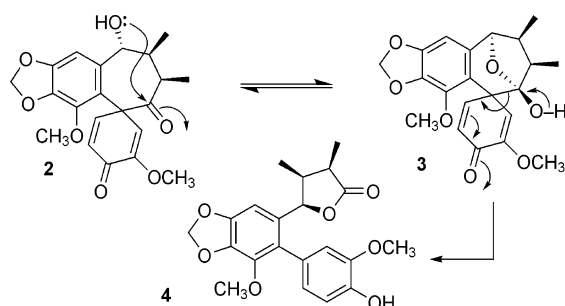
FIGURE 2. Rearrangement of the dimeric lignan skeleton. 3
