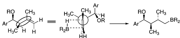
FIGURE 4. Diastereoselective hydroboration.
